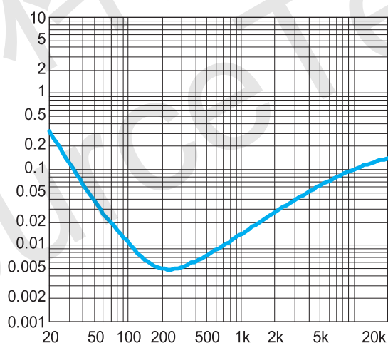
Figure 12. THD+N vs. Frequency SE mode, 3V, 32Ohm, Po=20mW
