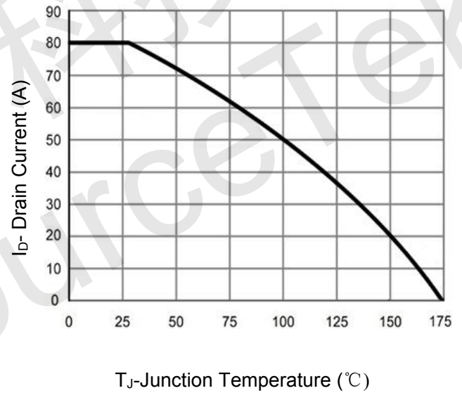
Figure 4 Drain Current
