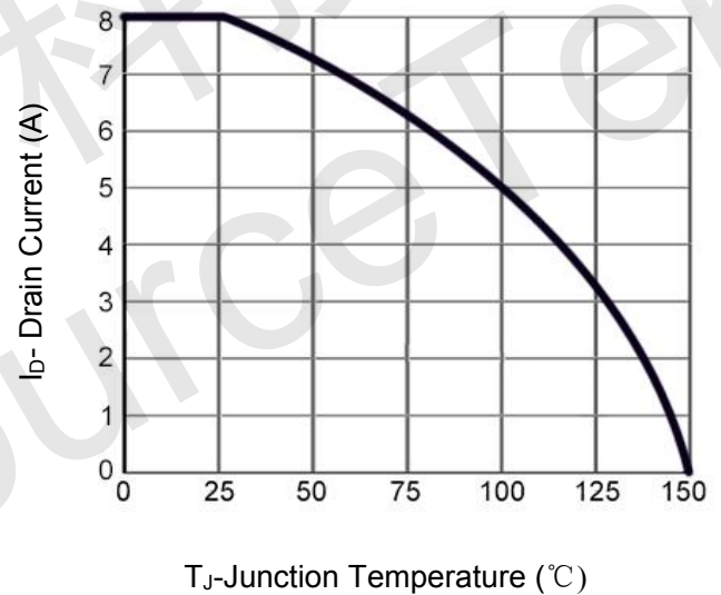
Figure 4 Drain Current
