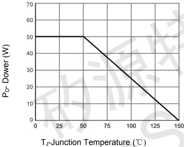
Figure 3 Power De-rating
