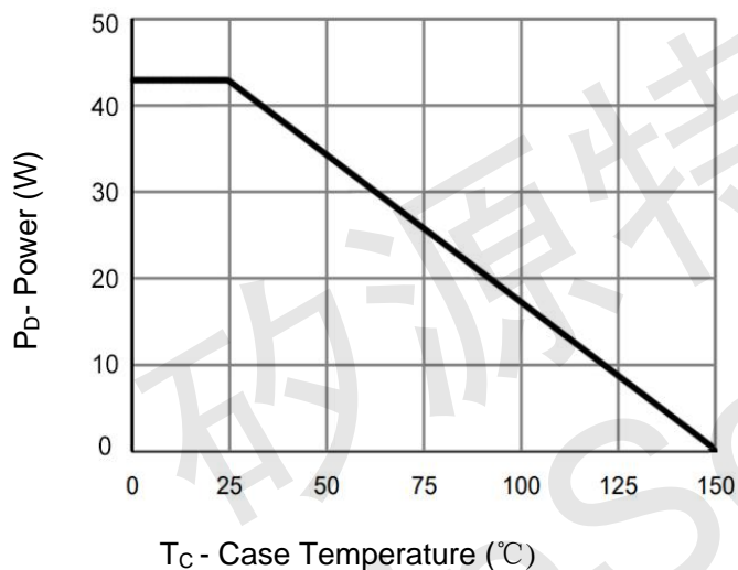
Figure 3 Power De-rating
