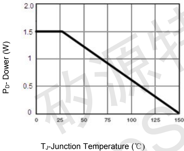
Figure 3 Power Dissipation
